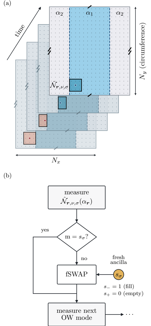
FIG. 1. Domain-wall geometry and adaptive circuit. (a) Four time slices illustrate OW updates in the periodic geometry, with \alpha_{\mathbf{r}} = \alpha_1 in the central slab and \alpha_2 in the trivial exterior. Along the time arrow, the supports progress from the exterior bulk through either side of the left interface to the slab bulk. Matching marks identify opposite boundaries. Salmon and blue windows show exterior and slab OW supports; dots mark their centers. Bulk supports contain 3 \times 3 cells; interface supports are clipped and renormalized. (b) An occupation measurement returns the Born outcome m . If m = s_{\sigma} , correction is bypassed; otherwise an fSWAP with a fresh ancilla restores s_- = 1 or s_+ = 0 . The branches rejoin and the procedure repeats for subsequent OW modes.
