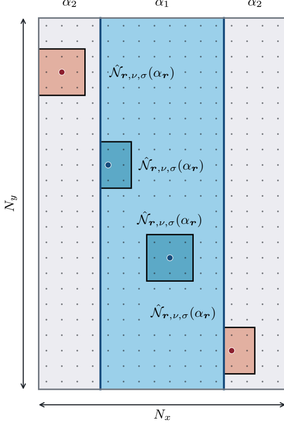
FIG. 1. Domain-wall geometry and local supports. A single N_x \times N_y cell, periodic in both directions, with a central slab ( \alpha_1 ) and trivial exterior ( \alpha_2 ). Four OW occupation measurements illustrate supports in the trivial bulk, at an interface on the slab side, in the slab bulk, and at an interface on the exterior side. Salmon and blue shading denote exterior and slab modes; dots mark their centers. Bulk supports contain 3 \times 3 unit cells. At the deep-blue interfaces, supports are clipped to the region containing their center and the surviving modes are renormalized.
