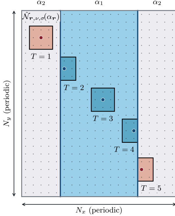
FIG. 1. Domain-wall geometry and local supports. A single N_x \times N_y cell, periodic in both directions, with a central slab ( \alpha_1 ) and trivial exterior ( \alpha_2 ). The lattice has five exterior columns on each side and ten slab columns. The labels T = 1, \dots, 5 identify example OW occupation measurements: in the trivial bulk, on the slab side of the left interface, in the slab bulk, on the slab side of the right interface, and on the exterior side of the right interface. The operator label shown once applies to all five supports. Salmon and blue shading denote exterior and slab modes; dots mark their centers. Bulk supports contain 3 \times 3 unit cells. At the deep-blue interfaces, supports are clipped to the region containing their center and the surviving modes are renormalized.
