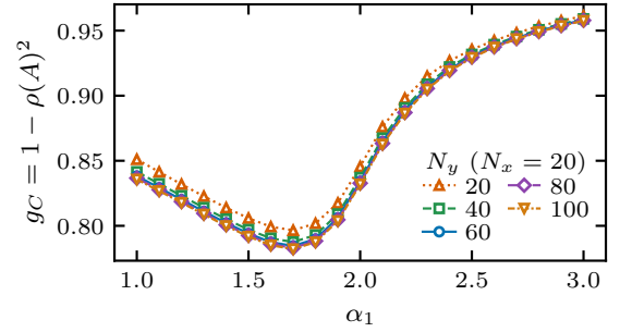
FIG. A4. Parameter dependence of the averaged-channel gap. Exact multiplier gap g_C = 1 - \rho(A)^2 for the fixed raster schedule at N_x = 20 and N_y = 20, 40, 60, 80, 100 . Each size uses 21 equally spaced values of \alpha_1 from 1 to 3, with \alpha_2 = 30 and hard-wall OW range w = 1 . These are deterministic one-cycle spectral calculations, with no sampled trajectories or statistical error bars. Lines connect sampled points as guides to the eye.
