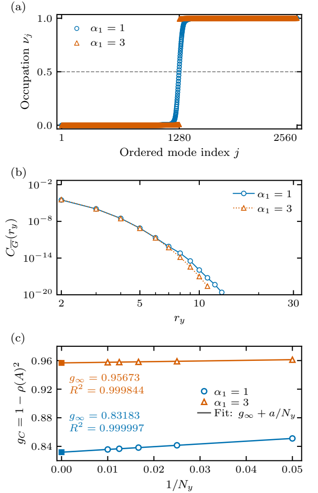
FIG. 10. Trajectory-averaged dynamics and channel gap. (a) Ordered occupation spectrum \nu_j of the trajectory-averaged two-point matrix \bar{G} , with every eigenvalue shown ( j = 1, \dots, 2N_x N_y ). Open blue circles and orange triangles denote \alpha_1 = 1 and 3 , respectively. (b) Squared correlation C_{\bar{G}}(r_y) of the same matrix. Both panels use N_x = 20 , N_y = 64 , after 128 cycles from maximal mixing. Panel (b) uses logarithmic axes for C_{\bar{G}}(r_y) versus r_y \geq 2 ; correlations below 10^{-20} are not displayed. (c) Fits of the multiplier gap g_C = 1 - \rho(A)^2 to g_\infty + a/N_y at \alpha_1 = 1, 3 , with fixed N_x = 20 and all five sizes N_y = 20, 40, 60, 80, 100 ; squares at 1/N_y = 0 mark extrapolated intercepts. Outcomes are averaged analytically in the fixed repeated raster schedule, so there is no sampled-trajectory count or SEM. The gap is dimensionless.
