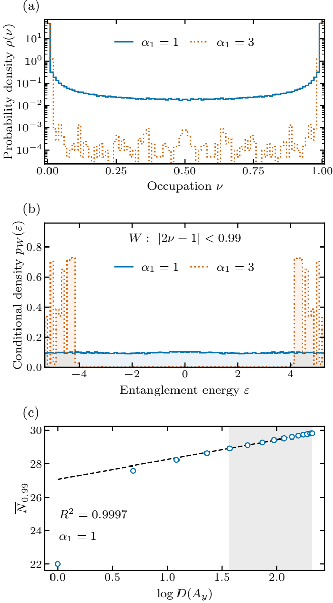
FIG. 7. Restricted spectra and mode count. Hard-wall states at N_x = 20 , N_y = 32 , cycle 64, from S = 100 independent random-pure half-filled trajectories per \alpha_1 = 1, 3 . (a) Full occupation histogram on 0 \leq \nu \leq 1 , normalized to unit area. (b) Conditional unit-area energy density for |2\nu - 1| < 0.99 , in 101 equal bins on [-\log 199, \log 199] . The central depletion at \alpha_1 = 3 contrasts with the finite near-zero density at \alpha_1 = 1 . Both histograms pool all 32 translated half-strips per trajectory. The retained totals are 95,398 and 83,326 for \alpha_1 = 1, 3 . (c) Raw mean window count for \alpha_1 = 1 , averaging origins within each trajectory. Bars are one trajectory SEM; the dashed fit uses 5 \leq A_y \leq 16 (shaded), while all widths are displayed. Translated cuts are correlated observations, not additional trajectories.
