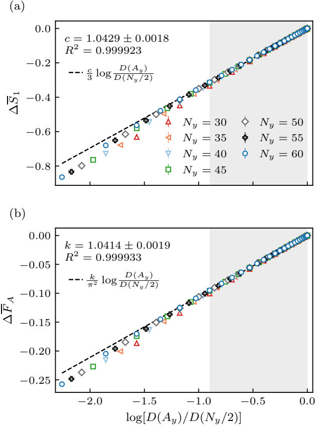
FIG. 6. Entanglement and charge fluctuations. (a) Mean strip entropy and (b) charge variance for N_y = 30, 35, \dots, 60 . The vertical-axis \Delta subtracts the value at A_y = \lfloor N_y/2 \rfloor ; the horizontal-axis reference D(N_y/2) uses the same rounded-down argument for odd N_y . Each case uses S = 100 independent random-pure half-filled trajectories after 2N_y cycles, with all strip origins averaged within each trajectory. Dashed lines are joint fits to Eq. (23) over 8 \leq A_y \leq \lfloor N_y/2 \rfloor (shaded). The point A_y = 1 is excluded from display only. The fits and their trajectory-based uncertainties retain correlations between strip widths.
