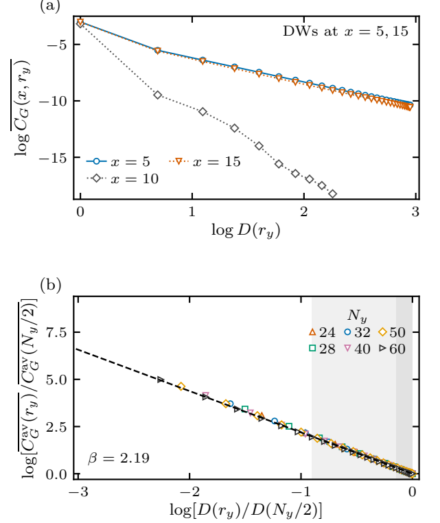
FIG. 5. Algebraic correlations on the walls. (a) Column-resolved correlations at \alpha_1 = 1 , N_y = 60 , for x = 5, 10, 15 . (b) Antipodally normalized correlations for N_y = 24, 28, 32, 40, 50, 60 , displaying r_y \geq 2 . The dashed line is a joint power-law fit over 8 \leq r_y \leq N_y/2 , with equal total weight per size and \beta \approx 2.19 . [Claude: General note on captions: many carry estimator details (“transformed through the absolute value”, “translated cuts are correlated observations”, “the gap is dimensionless”). Keep panel descriptions and parameters, and move statistics conventions to one sentence at the start of Sec. III, which you already have.] Gray shading marks the fit-window range. The data use S = 100 independent random-pure half-filled trajectories per case, observed after 2N_y cycles; spatial averaging precedes trajectory averaging, and the logarithm is taken last. Values below 10^{-8} are omitted from (a).
