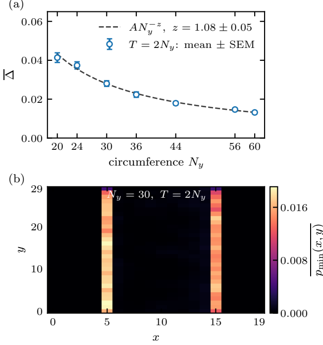
FIG. 4. Finite-time Lyapunov gap and boundary modes. (a) Mean gap at T = 2N_y for N_y = 20, 24, 30, 36, 44, 56, 60 ; the dashed line is an SEM-weighted fit over all seven sizes, with z = 1.08 \pm 0.05 . The slab is initially maximally mixed and the decoupled exterior is pure. (b) Mean density of the unique slowest mode at N_y = 30 , T = 60 , starting with the full system maximally mixed. Both ensembles use \alpha_1 = 1 and S = 100 independent trajectories. Each gap and mode density is evaluated within a trajectory before averaging; error bars are one trajectory SEM.
