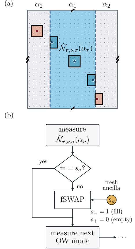
FIG. 1. Domain-wall geometry and adaptive circuit. (a) Periodic geometry with \alpha_{\mathbf{r}} = \alpha_1 in the central slab and \alpha_2 in the trivial exterior. Matching marks identify opposite boundaries. Salmon and blue windows show exterior and slab OW supports; dots mark their centers. Bulk supports contain 3 \times 3 cells; interface supports are clipped and renormalized. (b) An occupation measurement returns the Born outcome m . If m = s_\sigma , correction is bypassed; otherwise an fSWAP with a fresh ancilla restores s_- = 1 or s_+ = 0 . The branches rejoin and the procedure repeats for subsequent OW modes.
