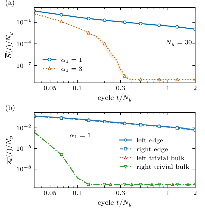
FIG. 3. Slow purification at the domain walls. (a) Mean entropy per unit length at N_y = 30 for \alpha_1 = 1, 3 . (b) Column entropy at \alpha_1 = 1 on the walls, x = 5, 15 , and in the trivial exterior, x = 2, 18 . Both panels start with the full system maximally mixed and use S = 100 independent trajectories evolved for 60 cycles. Bands are one trajectory SEM; the trivial entropy plateau is a numerical floor.
