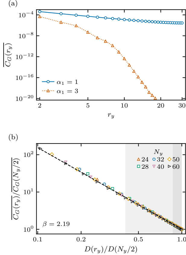
FIG. 5. Algebraic correlation scaling. (a) \overline{C_G}(r_y) versus separation r_y at N_y = 60 for \alpha_1 = 1 (circles, solid) and 3 (triangles, dotted); values at or below 10^{-20} are omitted. (b) Antipodally normalized correlations at \alpha_1 = 1 for N_y = 24, 28, 32, 40, 50, 60 , plotted against the normalized chord length. Both panels use logarithmic axes and display only r_y \geq 2 . The dashed line is the joint power-law fit over 8 \leq r_y \leq N_y/2 , with equal total weight per size and \beta \approx 2.19 ; light and darker gray mark the union and overlap of the size-dependent fit windows. Each ensemble contains S = 100 independent random-pure half-filled trajectories observed after 2N_y cycles, with N_x = 20 , \alpha_2 = 30 , and w = 1 . The squared correlator is averaged over position and trajectories before the normalization in (b). [Claude: General note on captions: many carry estimator details (“transformed through the absolute value”, “translated cuts are correlated observations”, “the gap is dimensionless”). Keep panel descriptions and parameters, and move statistics conventions to one sentence at the start of Sec. III, which you already have.]
