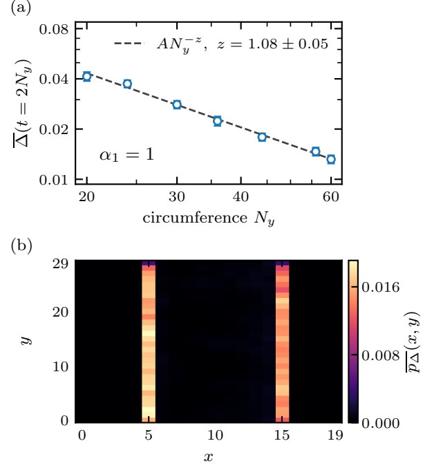
FIG. 4. Finite-time Lyapunov gap and boundary localization. (a) Mean gap \overline{\Delta}(t = 2N_y) for \alpha_1 = 1 and N_y = 20, 24, 30, 36, 44, 56, 60 at fixed N_x = 20 . The dashed line is an SEM-weighted fit over all seven sizes, with z = 1.08 \pm 0.05 ; error bars are one trajectory SEM. The slab is initially maximally mixed and the decoupled exterior is pure. (b) Mean spatial density of the unique slowest mode for \alpha_1 = 1 , N_y = 30 , and t = 60 , starting with the full system maximally mixed. Each panel uses S = 100 independent trajectories; gaps and normalized mode densities are evaluated per trajectory before averaging.
