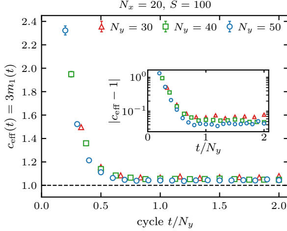
FIG. A3. Convergence of the entropy coefficient. Cycle dependence of c_{\text{eff}} = 3m_1 for N_x = 20 and N_y = 30, 40, 50 , from S = 100 independent random-pure trajectories per size evolved through 2N_y cycles. Strip origins are averaged within each trajectory, then trajectories are averaged before fitting \bar{S} versus log chord length with a free intercept over 8 \leq A_y \leq N_y/2 . Points show every fifth cycle from t = 10 ; bars are three times the regression standard error of the mean-curve slope. The inset resolves |c_{\text{eff}} - 1| on a logarithmic scale. The dashed horizontal reference is one.
