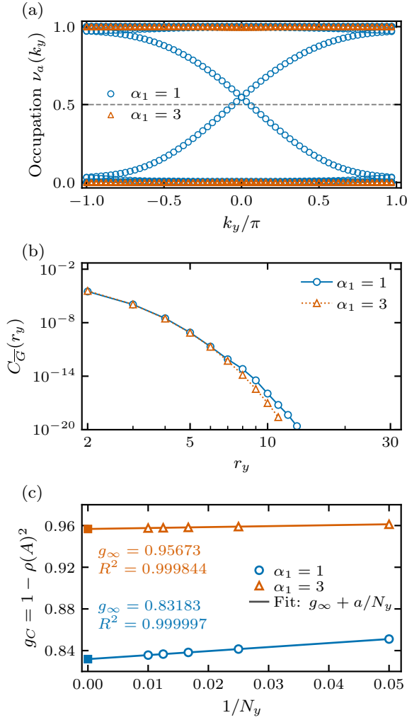
FIG. 10. Trajectory-averaged dynamics and channel gap. (a) Occupations of the translation-averaged two-point matrix and (b) its squared correlation at N_y = 64 , after 128 cycles from maximal mixing, for \alpha_1 = 1, 3 . Panel (b) uses logarithmic axes for C_{\bar{G}}(r_y) versus r_y \geq 2 ; correlations below 10^{-20} are not displayed. (c) Fits of the multiplier gap g_C = 1 - \rho(A)^2 to g_\infty + a/N_y at \alpha_1 = 1, 3 , with fixed N_x = 20 and all five sizes N_y = 20, 40, 60, 80, 100 ; squares at 1/N_y = 0 mark extrapolated intercepts. Outcomes are averaged analytically in the fixed repeated raster schedule, so there is no sampled-trajectory count or SEM. The gap is dimensionless.
