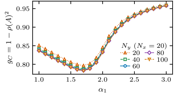
FIG. A4. Parameter dependence of the averaged-channel gap. Exact multiplier gap g_C = 1 - \rho(A)^2 for the fixed raster schedule at N_x = 20 and N_y = 20, 40, 60, 80, 100 . Each size uses 21 equally spaced values of \alpha_1 from 1 to 3, with \alpha_2 = 30 and hard-wall OW range w = 1 . These are deterministic one-cycle spectral calculations, with no sampled trajectories or statistical error bars. Lines connect sampled points as guides to the eye.
