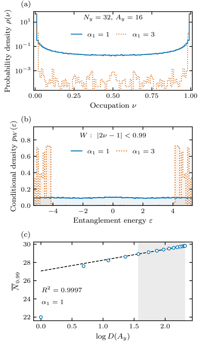
FIG. 7. Restricted spectra and mode count. Hard-wall states at N_x = 20, N_y = 32 , cycle 64, from S = 100 independent random-pure half-filled trajectories per \alpha_1 = 1, 3 . (a) Full occupation histogram on 0 \leq \nu \leq 1 , normalized to unit area. (b) Conditional unit-area energy density for |2\nu - 1| < 0.99 , in 101 equal bins on [-\log 199, \log 199] . The central depletion at \alpha_1 = 3 contrasts with the finite near-zero density at \alpha_1 = 1 . Both histograms pool all 32 translated half-strips per trajectory. The retained totals are 95,398 and 83,326 for \alpha_1 = 1, 3 . (c) Raw mean window count for \alpha_1 = 1 , averaging origins within each trajectory. Bars are one trajectory SEM; the dashed fit uses 5 \leq A_y \leq 16 (shaded), while all widths are displayed. Translated cuts are correlated observations, not additional trajectories.
