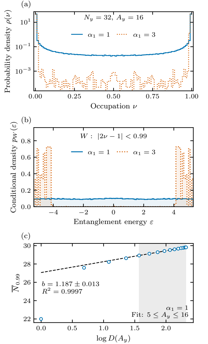
FIG. 6. Restricted spectra and mode count. Hard-wall states at N_x = 20 , N_y = 32 , cycle 64, from S = 100 independent random-pure half-filled trajectories per \alpha_1 = 1, 3 . (a) Full occupation histogram on 0 \leq \nu \leq 1 , normalized to unit area. (b) Conditional unit-area energy density for |2\nu - 1| < 0.99 , in 101 equal bins on [-\log 199, \log 199] . The central depletion at \alpha_1 = 3 contrasts with the finite near-zero density at \alpha_1 = 1 . Both histograms pool all 32 translated half-strips per trajectory. The retained totals are 95,398 and 83,326 for \alpha_1 = 1, 3 . (c) Raw mean window count for \alpha_1 = 1 , averaging origins within each trajectory. Bars are one trajectory SEM; the dashed fit uses 5 \leq A_y \leq 16 (shaded), while all widths are displayed. Translated cuts are correlated observations, not additional trajectories.
