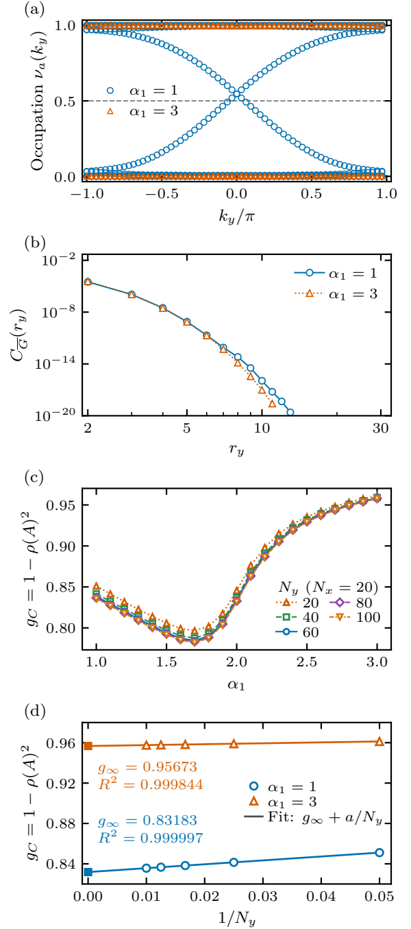
FIG. 9. Trajectory-averaged dynamics and channel gap. (a) Occupations of the translation-averaged two-point matrix and (b) its squared correlation at N_y = 64 , after 128 cycles from maximal mixing, for \alpha_1 = 1, 3 . Panel (b) uses logarithmic axes for C_{\bar{G}}(r_y) versus r_y \geq 2 ; correlations below 10^{-20} are not displayed. (c) Exact multiplier gap g_C = 1 - \rho(A)^2 versus \alpha_1 at fixed N_x = 20 and N_y = 20, 40, 60, 80, 100 . (d) Fits g_\infty + a/N_y at \alpha_1 = 1, 3 , using all five sizes; squares at 1/N_y = 0 mark extrapolated intercepts. Outcomes are averaged analytically in the fixed repeated raster schedule, so there is no sampled-trajectory count or SEM. The gap is dimensionless.
