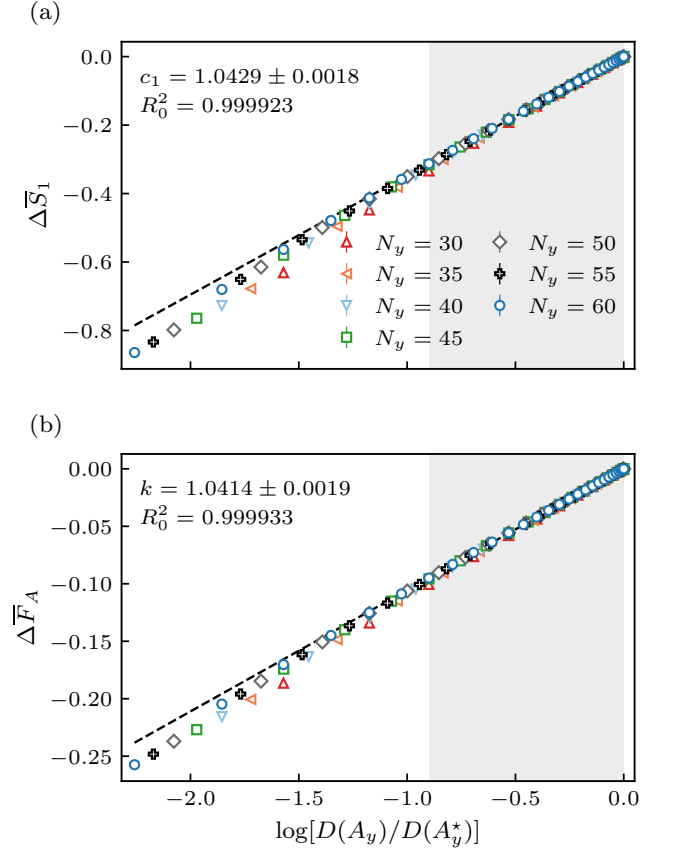
FIG. 5. Entanglement and charge fluctuations. (a) Mean strip entropy and (b) charge variance for N_y = 30, 35, \dots, 60 , shifted by their values at A_y = \lfloor N_y/2 \rfloor . Each case uses S = 100 independent random-pure half-filled trajectories after 2N_y cycles, with all strip origins averaged within each trajectory. Dashed lines are joint fits to Eq. (20) over 8 \leq A_y \leq \lfloor N_y/2 \rfloor (shaded). The point A_y = 1 is excluded from display only. The fits and their trajectory-based uncertainties retain correlations between strip widths.
