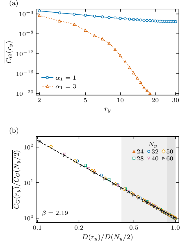
FIG. 4. Algebraic correlation scaling. (a) \overline{C}_G(r_y) versus separation r_y at N_y = 60 for \alpha_1 = 1 (circles, solid) and 3 (triangles, dotted); values at or below 10^{-20} are omitted. (b) Antipodally normalized correlations at \alpha_1 = 1 for N_y = 24, 28, 32, 40, 50, 60 , plotted against the normalized chord length. Both panels use logarithmic axes and display only r_y \geq 2 . The dashed line is the joint power-law fit over 8 \leq r_y \leq N_y/2 , with equal total weight per size and \beta \approx 2.19 ; light and darker gray mark the union and overlap of the size-dependent fit windows. Each ensemble contains S = 100 independent random-pure half-filled trajectories observed after 2N_y cycles, with N_x = 20 , \alpha_2 = 30 , and w = 1 . The squared correlator is averaged over position and trajectories before the normalization in (b). [Claude: General note on captions: many carry estimator details (“transformed through the absolute value”, “translated cuts are correlated observations”, “the gap is dimensionless”). Keep panel descriptions and parameters, and move statistics conventions to one sentence at the start of Sec. III, which you already have.]
