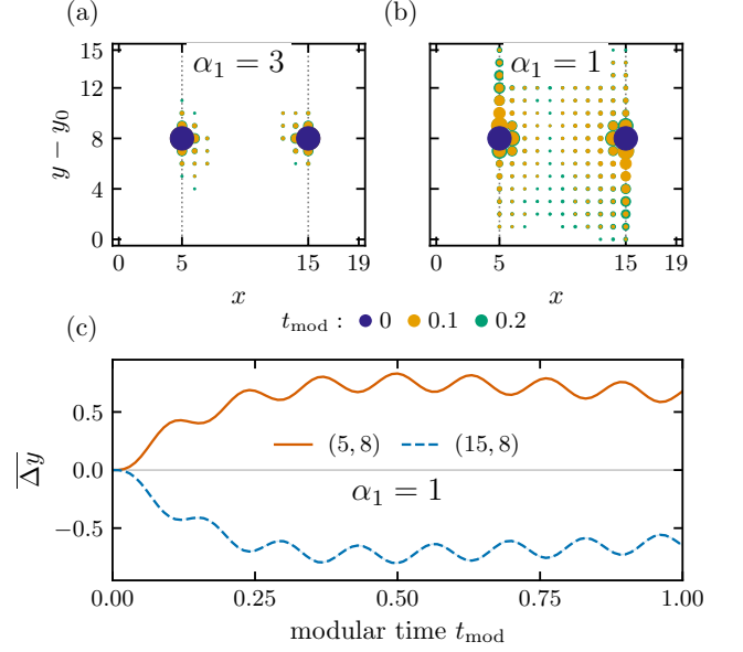
FIG. 8. Modular evolution on the walls. Two incoherent orbital profiles are initialized at each source cell (x, \delta y) = (5, A_y/2) or (15, A_y/2) in a half-cylinder of A_y = 16 rows. The states come from S = 100 independent random-pure trajectories per \alpha_1 = 1, 3 on a 20 \times 32 lattice after 64 cycles. (a,b) Mean densities at t_{\text{mod}} = 0, 0.1, 0.2 (purple, orange, green) for (a) \alpha_1 = 3 and (b) \alpha_1 = 1 . (c) Mean center-of-mass displacement \overline{\Delta y_{x_s}} from the initial row \delta y = A_y/2 , defined in Eq. (33), for \alpha_1 = 1 . Solid and dashed lines denote x_s = 5 and 15 ; each five-column window is normalized by its retained weight before averaging. Each observable is evaluated per cut, then averaged over 32 origins and trajectories. Bands are one trajectory SEM. Centered occupations are clipped at \pm(1 - 10^{-10}) when constructing h_A .
