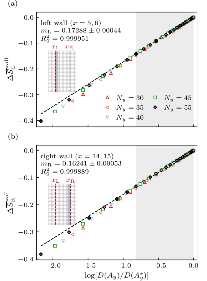
FIG. 7. Entropy carried by each wall. Entanglement contour integrated over (a) x = 5, 6 and (b) x = 14, 15 , for N_y = 30, 35, 40, 45, 55 . Each case uses S = 100 independent random-pure trajectories after 2N_y cycles. Contours are averaged over all translated strips within each trajectory before trajectory averaging, and anchored at A_y = \lfloor N_y/2 \rfloor . Dashed lines are joint fits over 8 \leq A_y \leq \lfloor N_y/2 \rfloor (shaded), with equal total weight per size and trajectory-based uncertainties including correlations between widths. Insets mark the integrated columns. The point A_y = 1 is omitted from display only.
