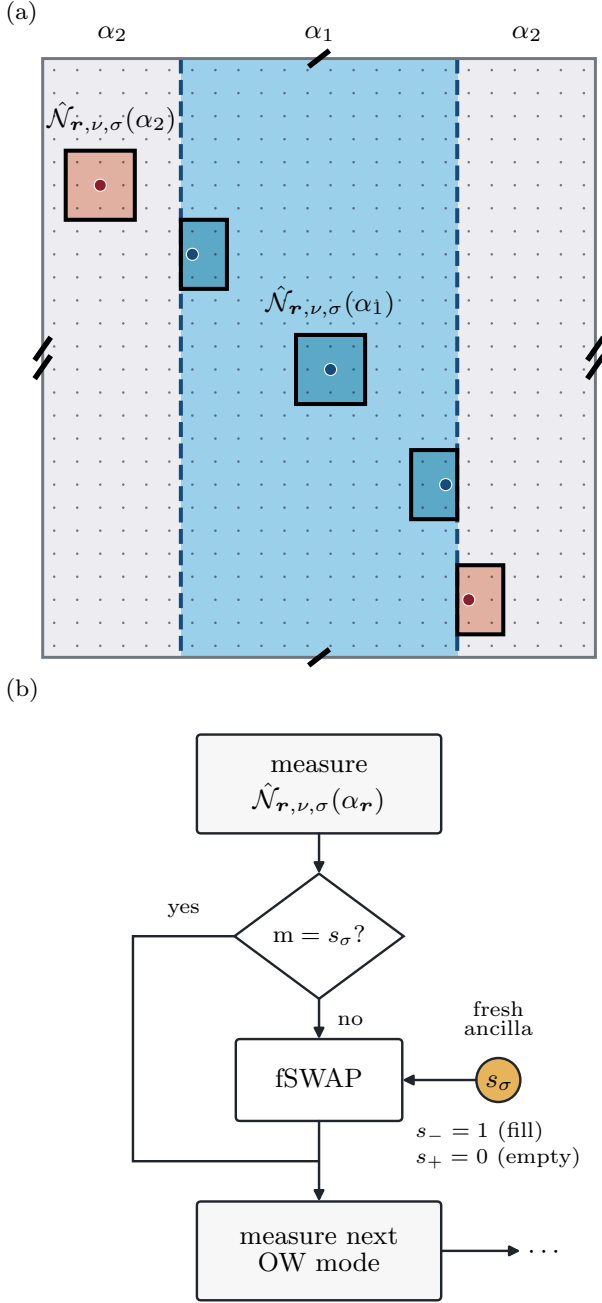
FIG. 1. Domain-wall geometry and adaptive circuit. (a) Periodic geometry with \alpha_{\mathbf{r}} = \alpha_1 in the central slab and \alpha_2 in the trivial exterior. Matching marks identify opposite boundaries. Salmon and blue windows show exterior and slab OW supports; dots mark their centers. Bulk supports contain 3 \times 3 cells; interface supports are clipped and renormalized. (b) An occupation measurement returns the Born outcome m . If m = s_{\sigma} , correction is bypassed; otherwise an fSWAP with a fresh ancilla restores s_- = 1 or s_+ = 0 . The branches rejoin and the procedure repeats for subsequent OW modes.
