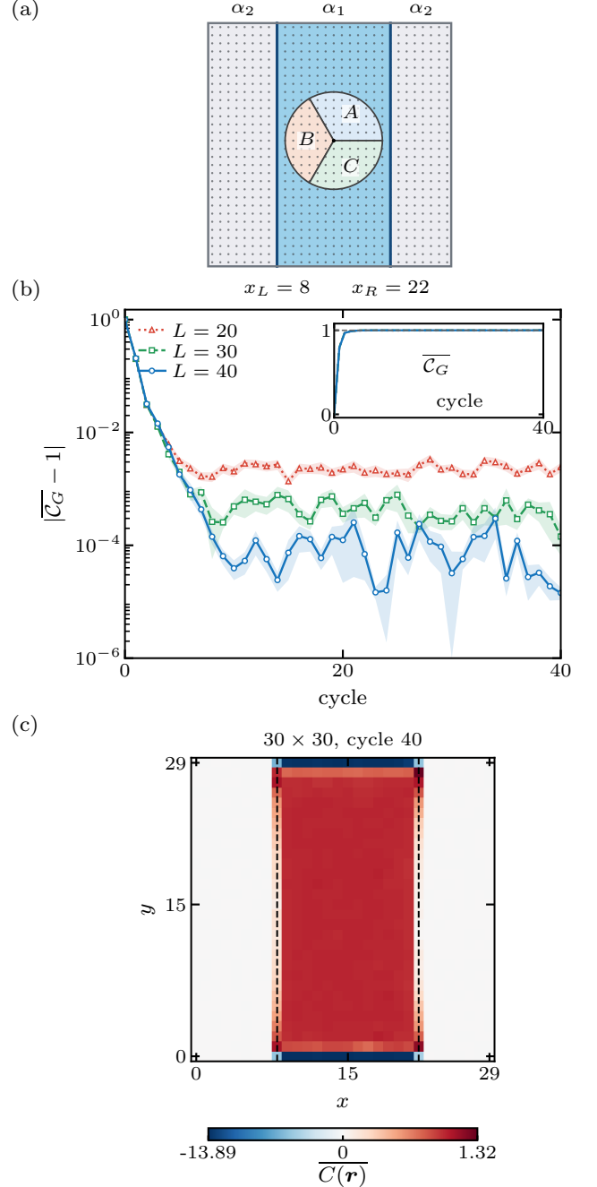
FIG. 2. Bulk topology in the domain-wall geometry.
