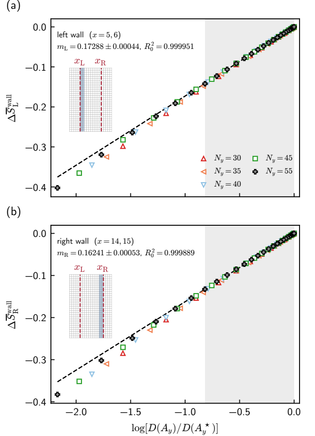
FIG. 9. Entropy carried by each wall. Entanglement contour integrated over (a) x = 5, 6 and (b) x = 14, 15 , for N_y = 30, 35, 40, 45, 55 . Each case uses S = 100 independent random-pure trajectories after 2N_y cycles. Contours are averaged over all translated strips within each trajectory before trajectory averaging, and anchored at A_y = \lfloor N_y/2 \rfloor . Dashed lines are joint fits over 8 \leq A_y \leq \lfloor N_y/2 \rfloor (shaded), with equal total weight per size and trajectory-based uncertainties including correlations between widths. Insets mark the integrated columns. The point A_y = 1 is omitted from display only.
