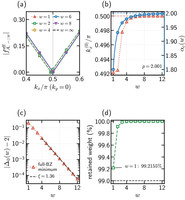
FIG. A1. Truncated OW modes at \alpha = 1 . (a) Effective form factor |f_{A,-;w}^{\text{eff}}| along k_y = 0 for w = 1, 2, 4, 6, 8, \infty . Symbols mark the zeros, and the dotted line marks the untruncated zero. (b) Position of the winding(-1) zero (red, left axis) and the critical parameter \alpha_c(w) of the truncated parent Hamiltonian (blue, right axis) with the fit of Eq. (A6). Dashed lines mark the w = \infty values. (c) Deviation of the half-filling gap \Delta_0(w) of the truncated parent Hamiltonian from its untruncated value, with an exponential fit for w \geq 4 . (d) Fraction of the squared OW norm retained inside the window.
