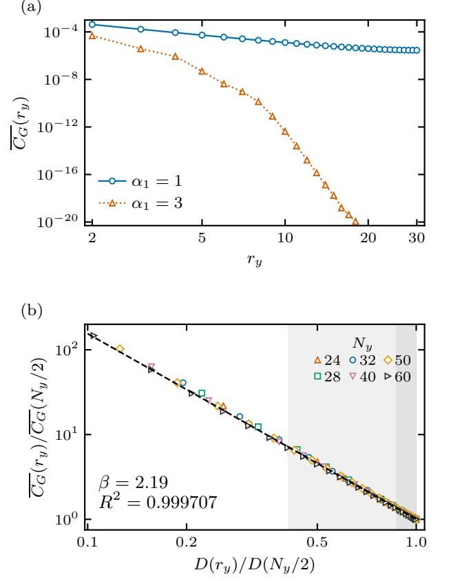
FIG. 5. Algebraic correlation scaling. (a) \bar{C}_G(r_y) versus separation r_y at N_y = 60 for \alpha_1 = 1 (circles, solid) and 3 (triangles, dotted); values at or below 10^{-20} are omitted. (b) Antipodally normalized correlations at \alpha_1 = 1 for N_y = 24, 28, 32, 40, 50, 60 , plotted against the normalized chord length. Both panels use logarithmic axes and display only r_y \geq 2 . The dashed line is the joint power-law fit over 8 \leq r_y \leq N_y/2 , with equal total weight per size and \beta \approx 2.19 ; light and darker gray mark the union and overlap of the size-dependent fit windows. Each ensemble contains S = 100 independent random-pure half-filled trajectories observed after 2N_y cycles, with N_x = 20 , \alpha_2 = 30 , and w = 1 . The squared correlator is averaged over position and trajectories before the normalization in (b). [Claude: General note on captions: many carry estimator details (“transformed through the absolute value”, “translated cuts are correlated observations”, “the gap is dimensionless”). Keep panel descriptions and parameters, and move statistics conventions to one sentence at the start of Sec. III, which you already have.]
