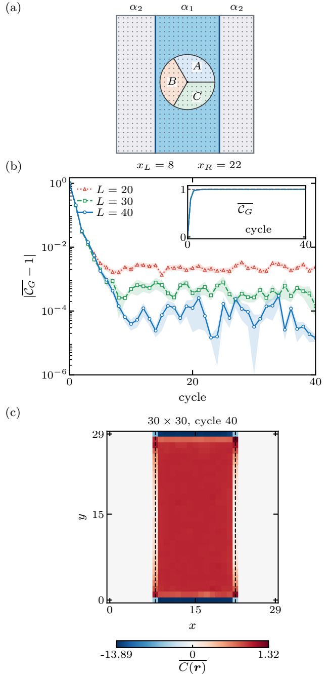
FIG. 3. Bulk topology in the domain-wall geometry.
