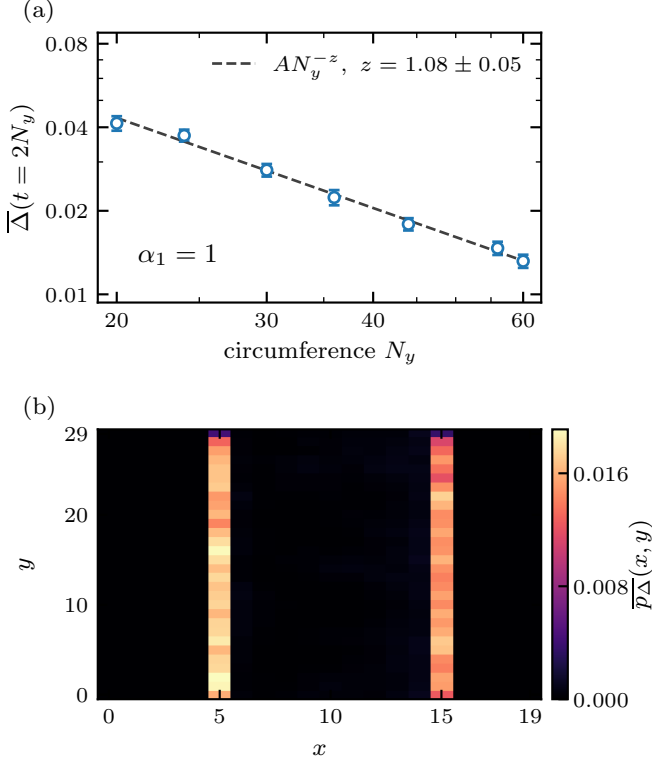
FIG. 4. Finite-time Lyapunov gap and boundary localization. (a) Mean gap \bar{\Delta}(t = 2N_y) for \alpha_1 = 1 and N_y = 20, 24, 30, 36, 44, 56, 60 at fixed N_x = 20 , on logarithmic axes. The dashed line is an SEM-weighted fit over all seven sizes, with z = 1.08 \pm 0.05 ; error bars are one trajectory SEM. The slab is initially maximally mixed and the decoupled exterior is pure. (b) Mean spatial density of the unique slowest mode for \alpha_1 = 1 , N_y = 30 , and t = 60 , starting with the full system maximally mixed. Each panel uses S = 100 independent trajectories; gaps and normalized mode densities are evaluated per trajectory before averaging.
