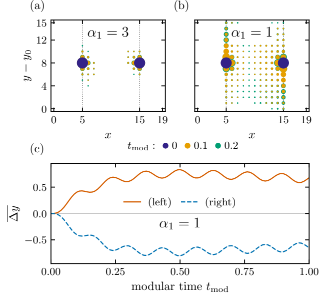
FIG. 10. Modular evolution on the walls. Two incoherent orbital profiles start at (x, \delta y) = (5, 8) or (15, 8) in a half-cylinder of 16 rows. The states come from S = 100 independent random-pure trajectories per \alpha_1 = 1, 3 , on a 20 \times 32 lattice after 64 cycles. (a,b) Mean densities at t_{\text{mod}} = 0, 0.1, 0.2 (purple, orange, green) for \alpha_1 = 3, 1 . (c) Mean displacement defined in Eq. (31) for \alpha_1 = 1 ; solid and dashed lines denote x_s = 5, 15 . Bands are one trajectory SEM.
