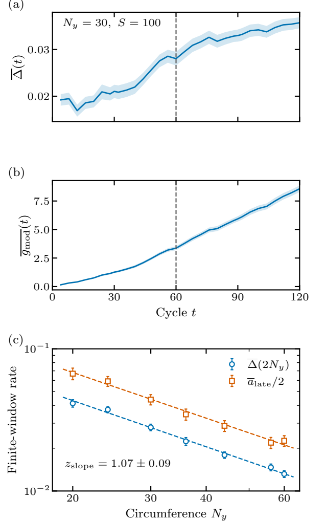
FIG. A2. Finite-time purification and raw-gap growth. (a) Mean rate \bar{\Delta}(t) and (b) mean raw modular gap \bar{g}_{\text{mod}}(t) for N_x = 20 , N_y = 30 , \alpha_1 = 1 , \alpha_2 = 30 , and w = 1 , through 120 cycles. The saved slab-only protocol starts with a maximally mixed slab and a Born-prepared pure exterior; S = 100 independent trajectories. The minimum is taken within each trajectory before averaging. Bands are one trajectory SEM; the vertical reference marks 2N_y . (c) Seven-size comparison of \bar{\Delta}(2N_y) with half the mean raw-gap secant slope over [3N_y, 4N_y] , defined in Eq. (C2). Bars are trajectory SEMs, with endpoint differences formed within each trajectory. Dashed lines are SEM-weighted power-law fits over all seven sizes; the displayed slope exponent has a formal regression error. The growth rate is a finite-window diagnostic, not an established asymptotic gap.
