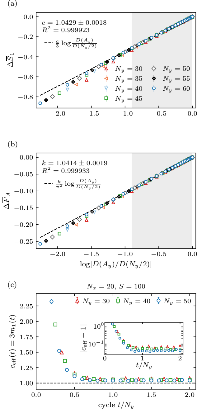
FIG. 6. Entanglement and charge fluctuations. (a) Mean strip entropy and (b) charge variance for N_y = 30, 35, \dots, 60 , from S = 100 independent random-pure half-filled trajectories after 2N_y cycles per size. The vertical-axis \Delta subtracts the half-strip value; D(N_y/2) uses the same rounded-down argument for odd N_y . Dashed lines are joint fits to Eq. (23) over 8 \leq A_y \leq \lfloor N_y/2 \rfloor (shaded). Bars and fit errors in (a,b) are trajectory SEMs; A_y = 1 is omitted from display only. (c) Saved c_{\text{eff}} = 3m_1 convergence for N_x = 20 , N_y = 30, 40, 50 , with S = 100 independent random-pure trajectories per size through 2N_y cycles. Mean entropy curves are fit with a free intercept over 8 \leq A_y \leq N_y/2 ; points show every fifth cycle from t = 10 , with bars equal to three times the slope's regression standard error. The inset shows |c_{\text{eff}} - 1| on a logarithmic axis.
