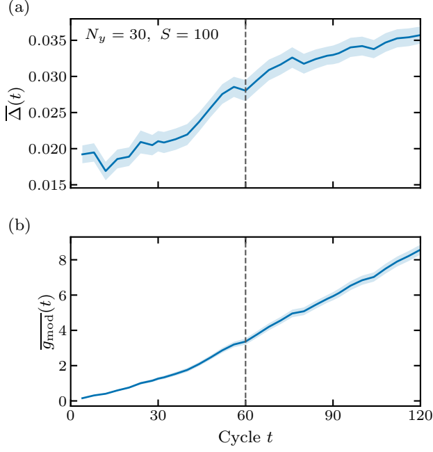
FIG. A2. Fixed-size purification diagnostic. (a) Mean finite-time rate \overline{\Delta}(t) and (b) mean raw modular gap \overline{g_{\text{mod}}}(t) for N_x = 20 , N_y = 30 , \alpha_1 = 1 , \alpha_2 = 30 , and w = 1 , through 120 cycles. The saved slab-only protocol starts with a maximally mixed slab and a Born-prepared pure exterior; S = 100 independent trajectories. The minimum is taken within each trajectory before averaging. Bands are one trajectory SEM; the vertical reference marks 2N_y . No time fit or extrapolation is shown.
