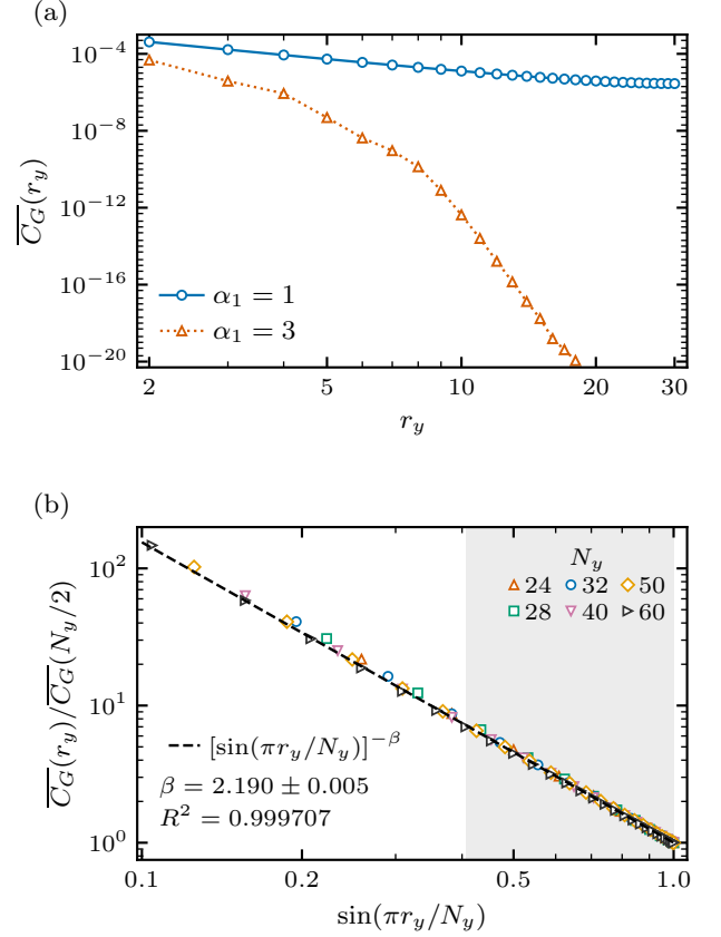
FIG. 5. Algebraic correlation scaling. (a) \overline{C}_G(r_y) at N_y = 60 for \alpha_1 = 1 (circles) and 3 (triangles). (b) Antipodally normalized correlations for \alpha_1 = 1 , N_y = 24, 28, 32, 40, 50, 60 , versus \sin(\pi r_y/N_y) . Both panels use logarithmic axes and show r_y \geq 2 ; values at or below 10^{-20} are omitted in (a). The dashed line is a joint power-law fit over 8 \leq r_y \leq N_y/2 , with equal total weight per size and \beta = 2.190 \pm 0.005 (regression error). Gray shading shows the union of fit windows. Each size uses S = 100 independent random-pure half-filled trajectories after 2N_y cycles, with N_x = 20 , \alpha_2 = 30 , and w = 1 .
