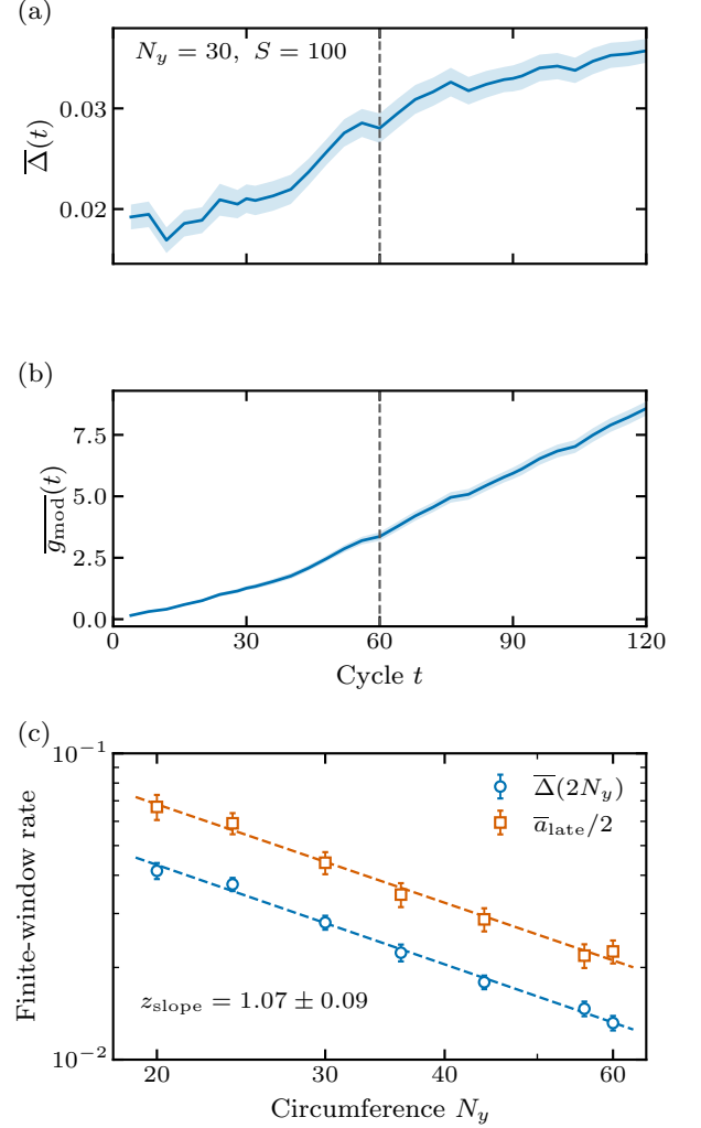
FIG. A2. Finite-time purification and raw-gap growth. (a) Mean rate \bar{\Delta}(t) and (b) mean raw modular gap \bar{g}_{\text{mod}}(t) for N_x = 20 , N_y = 30 , \alpha_1 = 1 , \alpha_2 = 30 , and w = 1 , through 120 cycles. The saved slab-only protocol starts with a maximally mixed slab and a Born-prepared pure exterior; S = 100 independent trajectories. The minimum is taken within each trajectory before averaging. Bands are one trajectory SEM; the vertical reference marks 2N_y . (c) Seven-size comparison of \bar{\Delta}(2N_y) with half the mean raw-gap secant slope over [3N_y, 4N_y] , defined in Eq. (C2). Bars are trajectory SEMs, with endpoint differences formed within each trajectory. Dashed lines are SEM-weighted power-law fits over all seven sizes; the displayed slope exponent has a formal regression error. The growth rate is a finite-window diagnostic, not an established asymptotic gap.
