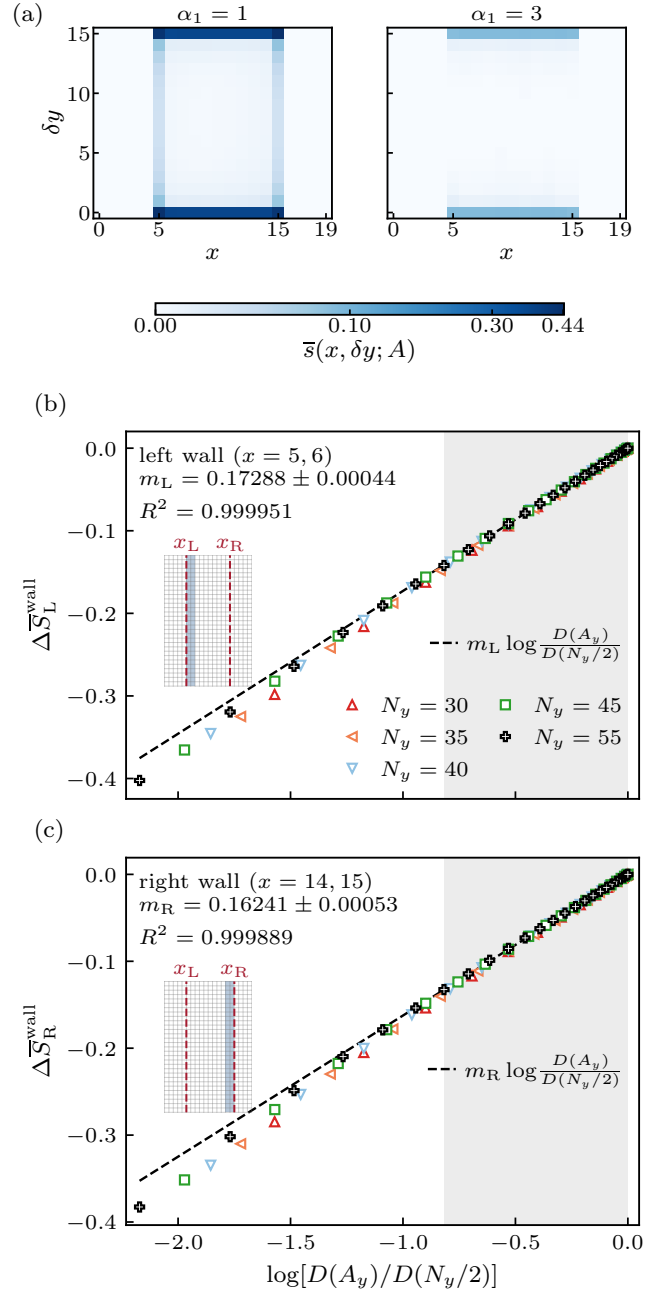
FIG. 8. Spatial entanglement and entropy carried by each wall. (a) Mean half-strip contours at N_x = 20 , N_y = 32 , cycle 64 for \alpha_1 = 1, 3 , on a shared square-root color scale; \delta y is relative to the strip origin. (b,c) Contour weight in columns x = 5, 6 and x = 14, 15 at \alpha_1 = 1 , for N_y = 30, 35, 40, 45, 55 after 2N_y cycles. Each ensemble uses S = 100 independent random-pure half-filled trajectories. The vertical-axis \Delta subtracts the half-strip value; D(N_y/2) denotes D(\lfloor N_y/2 \rfloor) for odd N_y . Dashed lines are joint fits over 8 \leq A_y \leq \lfloor N_y/2 \rfloor (shaded), with equal total weight per size. Bars and fit errors are trajectory SEMs. Insets mark the integrated columns; A_y = 1 is omitted from display only.
