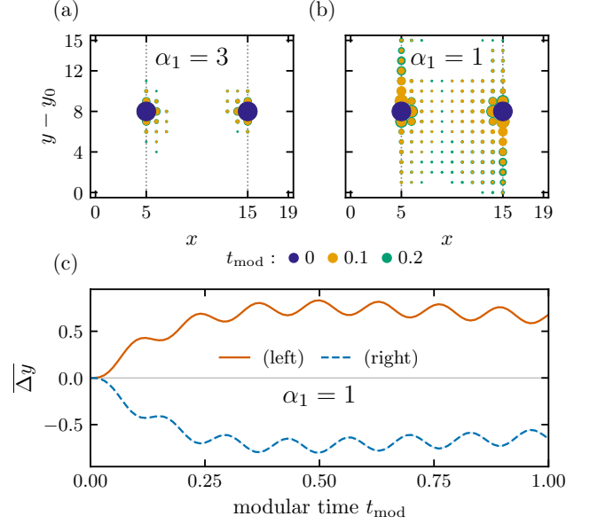
FIG. 9. Modular evolution on the walls. Two incoherent orbital profiles start at (x, \delta y) = (5, 8) or (15, 8) in a half-cylinder of 16 rows. The states come from S = 100 independent random-pure trajectories per \alpha_1 = 1, 3 , on a 20 \times 32 lattice after 64 cycles. (a,b) Mean densities at t_{\text{mod}} = 0, 0.1, 0.2 (purple, orange, green) for \alpha_1 = 3, 1 . (c) Mean displacement defined in Eq. (29) for \alpha_1 = 1 ; solid and dashed lines denote x_s = 5, 15 . Bands are one trajectory SEM.
