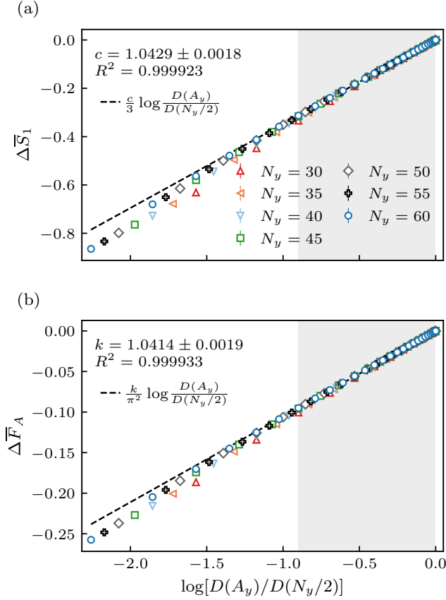
FIG. 6. Entanglement and charge fluctuations. (a) Mean strip entropy and (b) charge variance for N_y = 30, 35, \dots, 60 , from S = 100 independent random-pure half-filled trajectories after 2N_y cycles per size. The vertical-axis \Delta subtracts the half-strip value; D(N_y/2) uses the same rounded-down argument for odd N_y . Dashed lines are joint fits to Eq. (22) over 8 \leq A_y \leq \lfloor N_y/2 \rfloor (shaded). Bars and fit errors are trajectory SEMs. The point A_y = 1 is omitted from display only.
