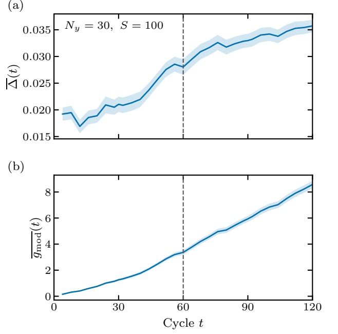
FIG. A2. Fixed-size purification diagnostic. (a) Mean finite-time rate \bar{\Delta}(t) and (b) mean raw modular gap g_{\text{mod}}(t) for N_x = 20 , N_y = 30 , \alpha_1 = 1 , \alpha_2 = 30 , and w = 1 , through 120 cycles. The saved slab-only protocol starts with a maximally mixed slab and a Born-prepared pure exterior; S = 100 independent trajectories. The minimum is taken within each trajectory before averaging. Bands are one trajectory SEM; the vertical reference marks 2N_y . No time fit or extrapolation is shown.
