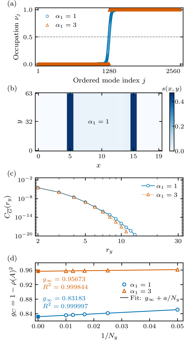
FIG. 1. Outcome-averaged hard-wall channel. (a) Endpoint occupation spectra for \alpha_1 = 1, 3 . (b) Full-system entropy contour s(x, y) for \alpha_1 = 1 , in nats per unit cell. (c) Squared averaged correlator. Panels (a)–(c) use the untwirled endpoints at cycle 128, starting from maximal mixing, with N_x = 20 , N_y = 64 and n_{\text{shell}} = 1 ; outcomes are averaged analytically. (d) Channel gap g_C = 1 - \rho(A)^2 at fixed N_x = 20 and varying N_y ; lines are the saved g_\infty + a/N_y fits. This caption is for layout assessment only.
