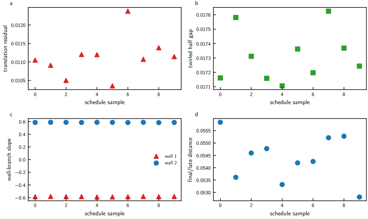
FIG. 2. Ten independent random schedules at the canonical channel endpoint. The raw translation residual ranges from 0.01035 to 0.01237, while the twirled midpoint gap is 0.01731 \pm 0.00018 . Wall slopes are stable, s_1 = -0.58513 \pm 0.00272 and s_2 = +0.58647 \pm 0.00152 , even though the final-to-late distance remains 0.05439 \pm 0.00095 . Uncertainties are sample standard deviations over the ten schedules.
