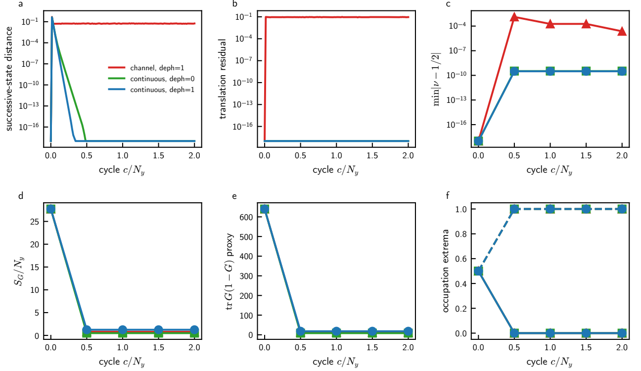
FIG. 1. Cycle diagnostics for the canonical N_y = 64 , n_{\text{shell}} = 1 , DW-truncated endpoint. The continuous arms reach machine-level successive-state and translation residuals by approximately c/N_y = 0.5 . The random ordered channel retains a nonzero cycle-to-cycle distance and translation residual, so its reported stationary spectrum is explicitly based on the late temporal average and translation twirl. The remaining panels show checkpoint midpoint gap, Gaussian entropy and charge-variance proxies, and occupation extrema.
