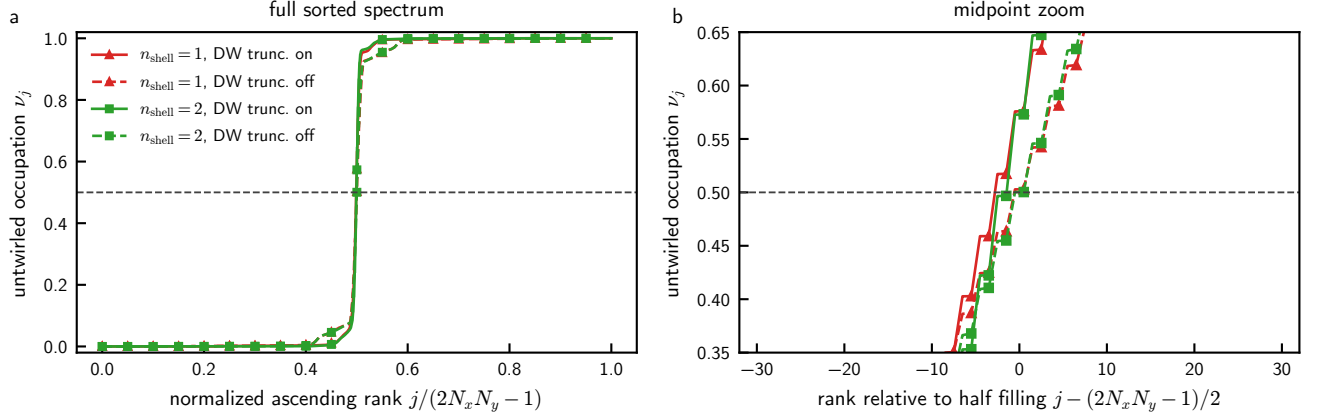
FIG. 2. Ascending natural occupations of the raw, untwirled channel late average \bar{G}_s at 20 \times 64 and \alpha_{\text{run}, \text{in}} = 1 . No translation twirl and no k_y block diagonalization is used. The left panel contains all 2N_xN_y = 2560 eigenvalues; the right panel magnifies the ranks nearest half filling. Color distinguishes n_{\text{shell}} = 1, 2 , and solid/dashed lines distinguish DW-support truncation on/off. These curves are global rank spectra, not dispersions.
