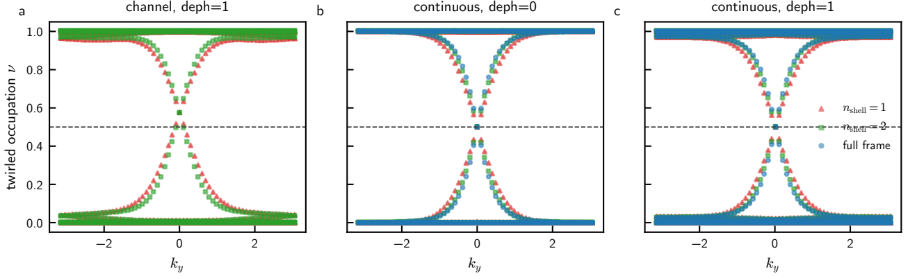
FIG. 1. Canonical k_y -resolved natural occupations at N_x \times N_y = 20 \times 64 , \alpha_{\text{run}, \text{in}} = 1 , \alpha_{\text{run}, \text{out}} = 30 , maximal-mixing initialization, and DW-support truncation on. Red triangles and green squares are n_{\text{shell}} = 1, 2 ; blue circles are the continuous full-frame control. The channel panel is the exact translation twirl of the cycle-65–128 average for one matched random schedule; continuous panels use exact k_y blocks over the corresponding time window. The dashed line marks \nu = 1/2 .
