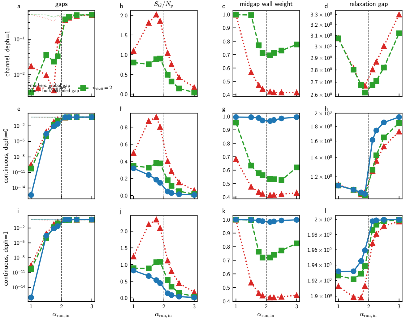
FIG. 3. Matched alpha scan at N_y = 64 with DW-support truncation on. Columns report the global (markers) and bulk-excluded (faint curves) midpoint gaps, S_G/N_y , midgap wall localization, and relaxation. The vertical line at \alpha_{\text{run},\text{in}} = 2 is a parent-model reference, not a sampled point. Rows are the full-dephasing channel, continuous no-dephasing evolution, and continuous full-dephasing evolution; colors/markers distinguish shell range.
