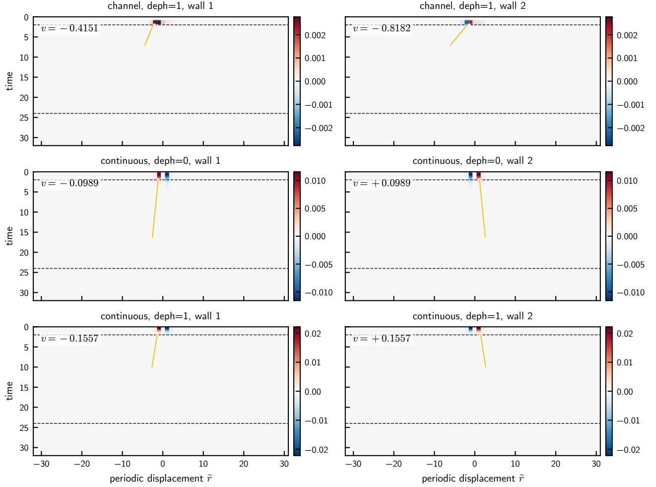
FIG. 4. Local density-phase response for the canonical N_y = 64 , n_{\text{shell}} = 1 , DW-truncated endpoint. Rows compare the channel and the two continuous arms; columns are the two walls. The channel stores all 64 source origins and is source-averaged only for display; exact translation symmetry makes one source sufficient in the continuous arms. White points and gold lines show the retained positive-lobe centers and OLS fits; dashed lines mark the nominal fit window. Displayed annotations are profile slopes, while source-resolved channel fit quality is reported in the text.
