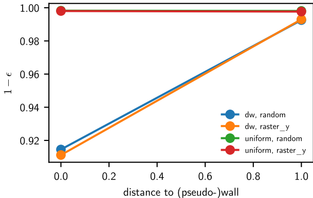
Constraint retention
