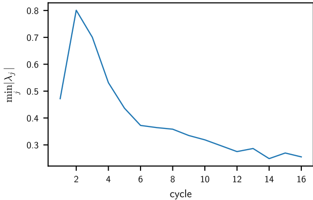
Lyapunov gap proxy
