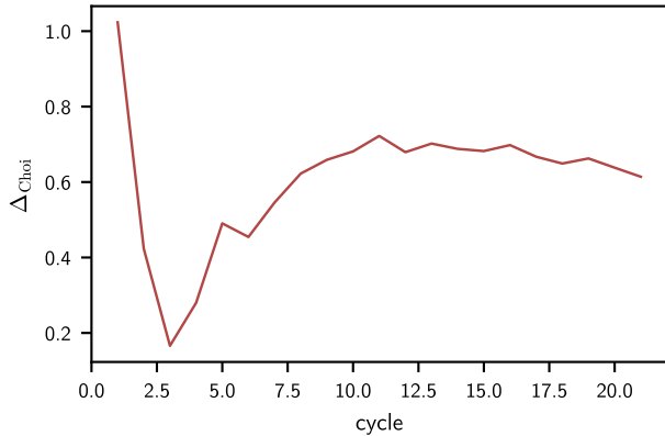
Regularized-Choi proxy
