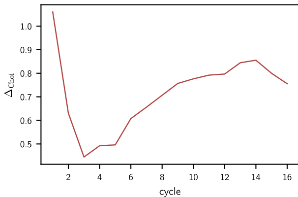
Regularized-Choi proxy
