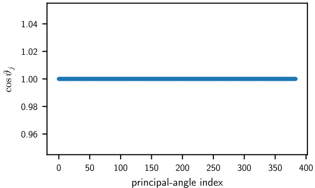
Controller-span overlap
