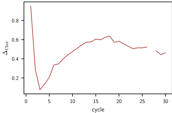
Regularized-Choi proxy
