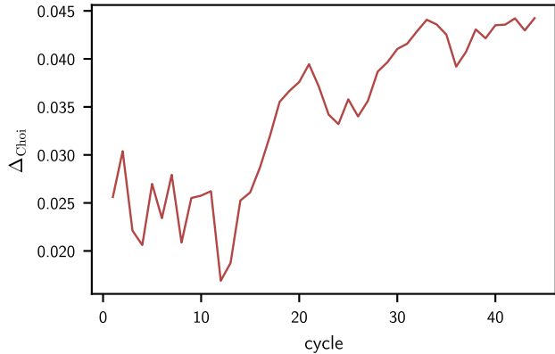
Regularized-Choi proxy
