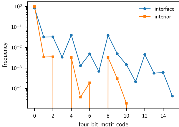
Raster-y motif population
