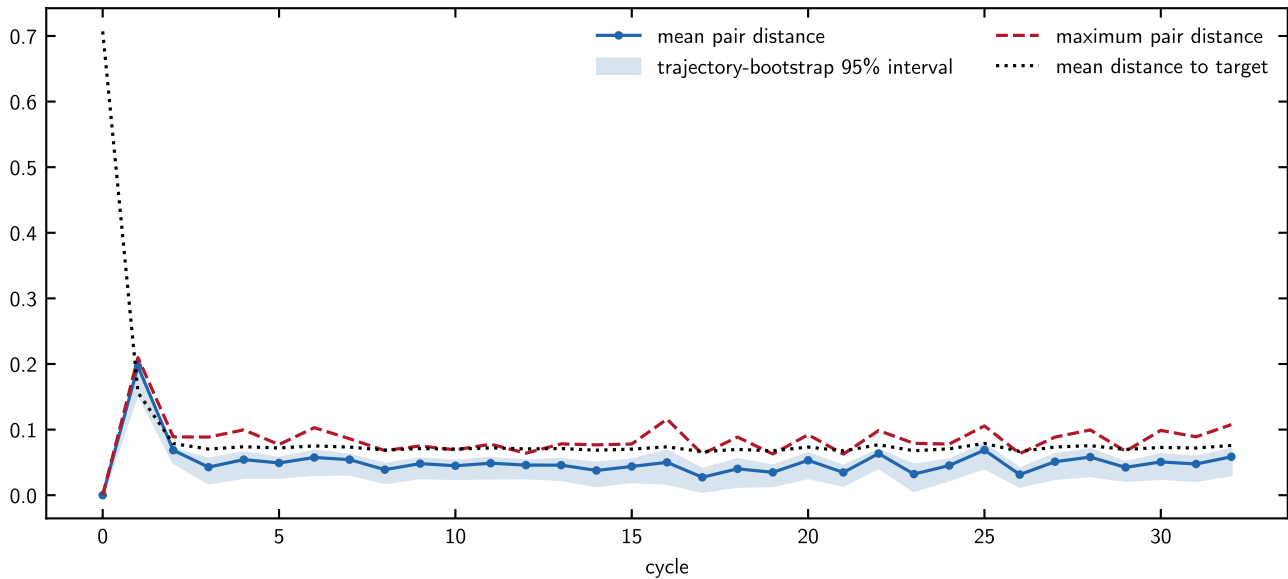
normalized projector distance
