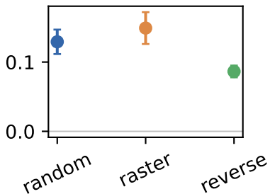
charge
