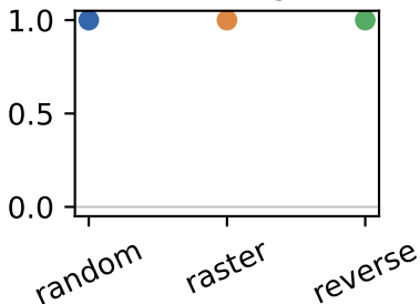
wall weight
