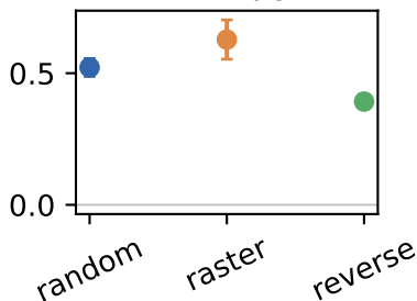
entropy
