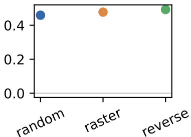
bulk C
