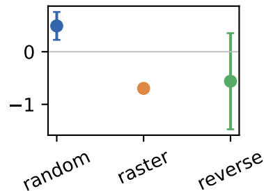
v right
