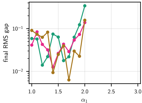
finite-only
