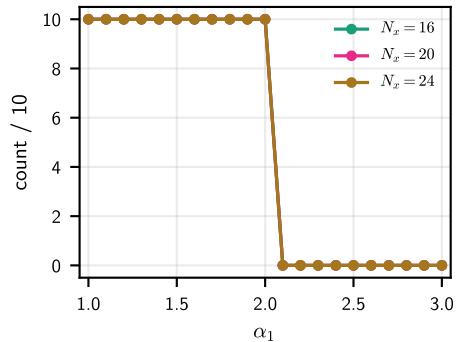
finite samples
