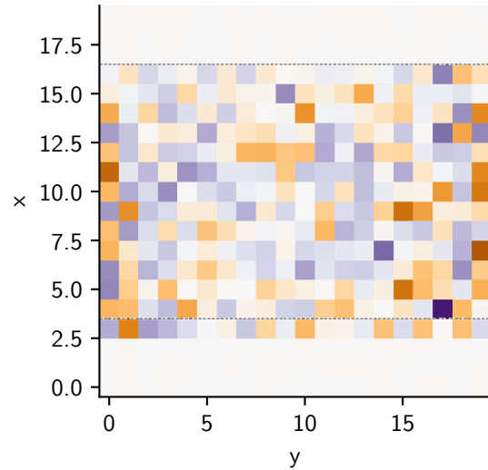
DW alpha=1/30, dwtrunc=0
