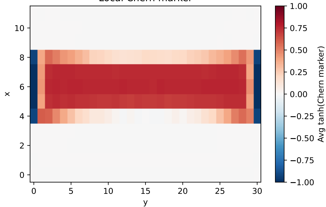
Local Chern marker
