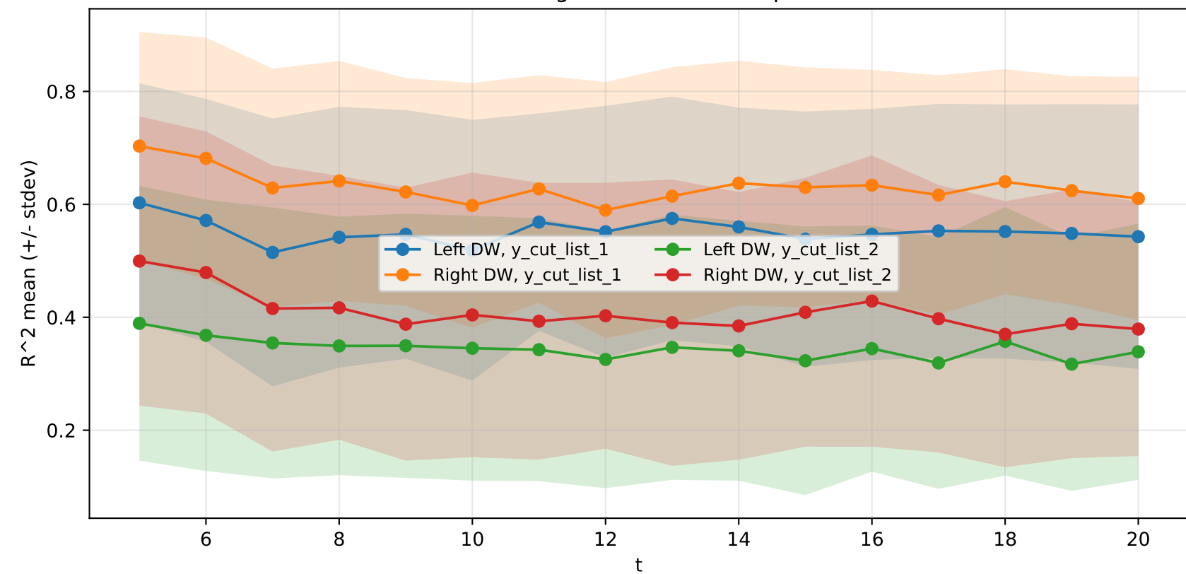
Average R^2 vs time-step
