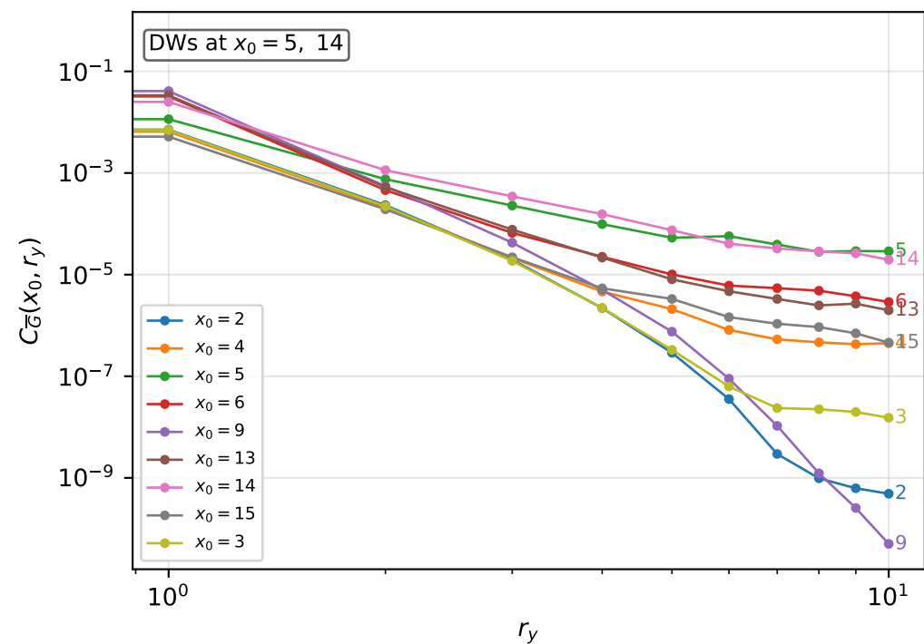
Correlation profiles &amp; spectra (cycles=20, samples=10)
