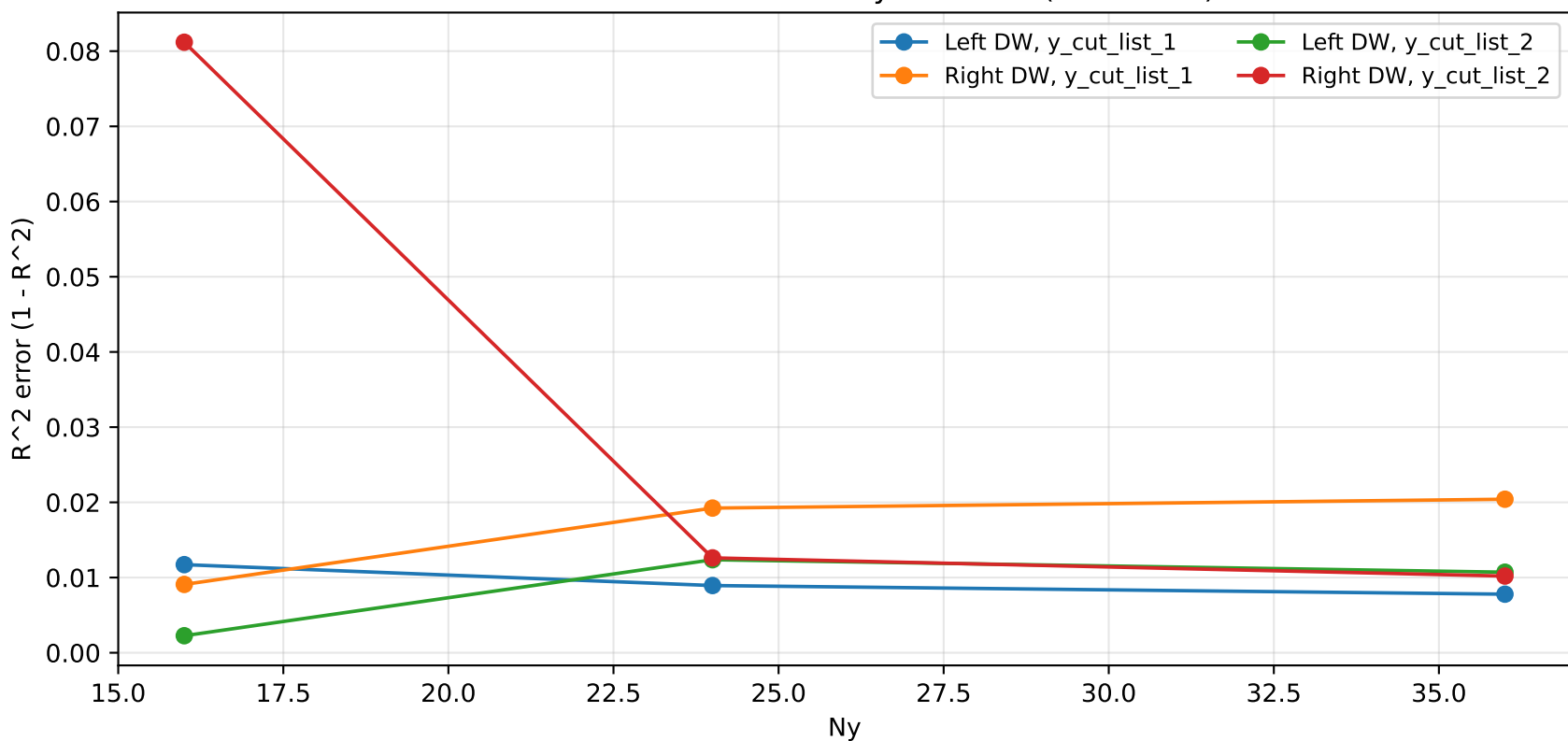
Post-selected: fit error vs system size (final state)
