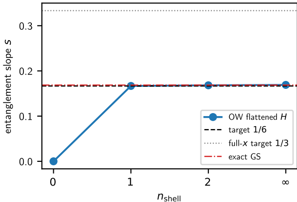
Entanglement contour slope vs. n_{\text{shell}}
