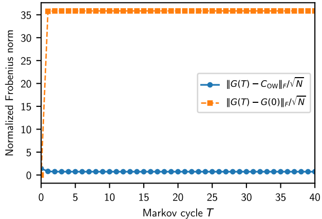
Post-selected (DW-trunc)
