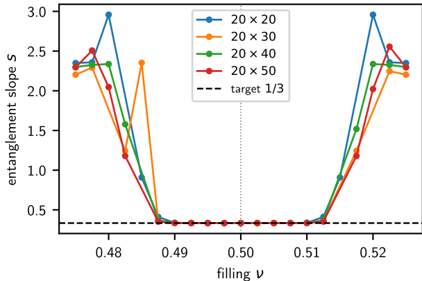
Entanglement slope vs. filling ( n_{\text{shell}} = 1 )
