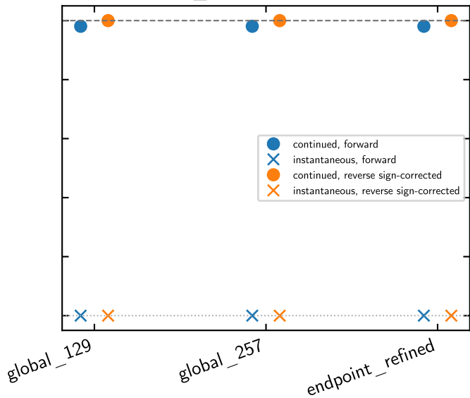
dw_truncation=True
