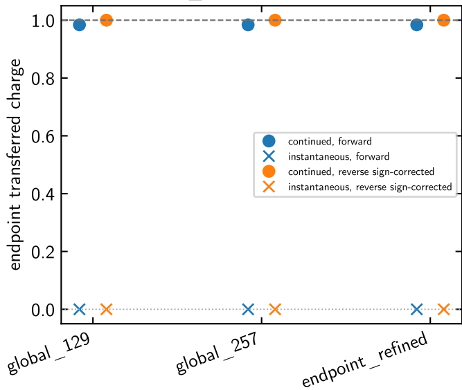
dw_truncation=False
