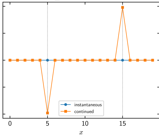
dw_truncation=True
