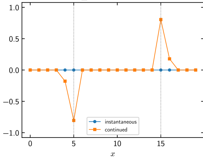
dw_truncation=False
