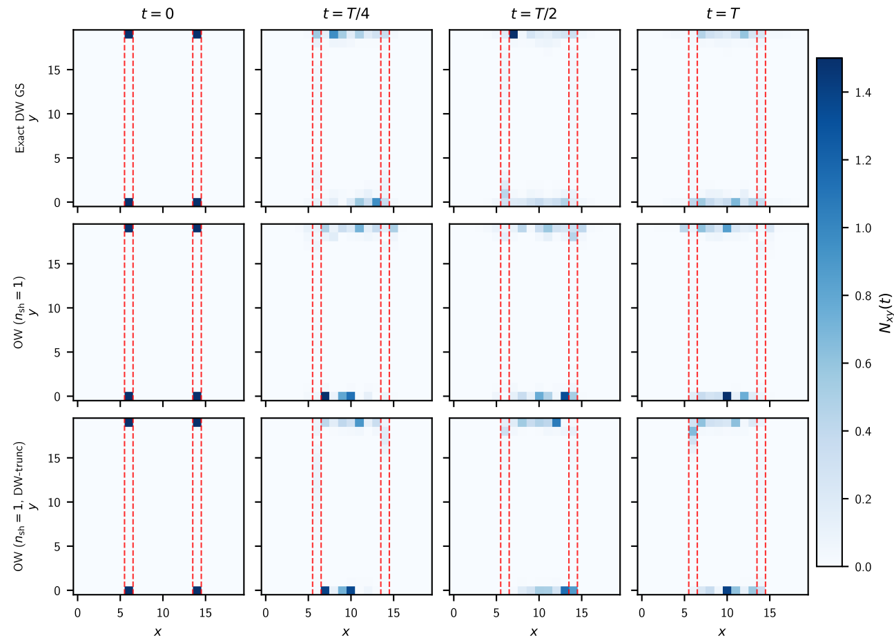
Charge density N_{xy}(t) snapshots (config 1)
