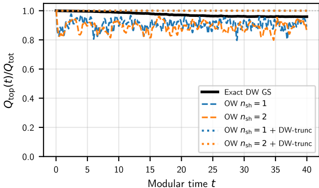
Topological charge fraction vs. modular time
