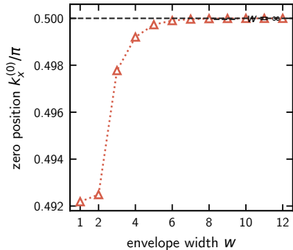
(a) zero at \alpha = 1, k_y = 0
