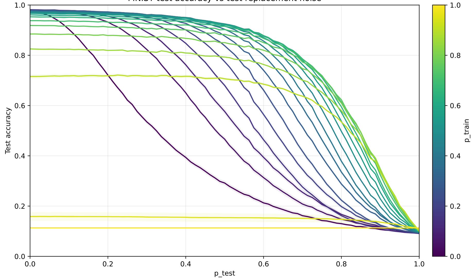
MNIST test accuracy vs test replacement noise
