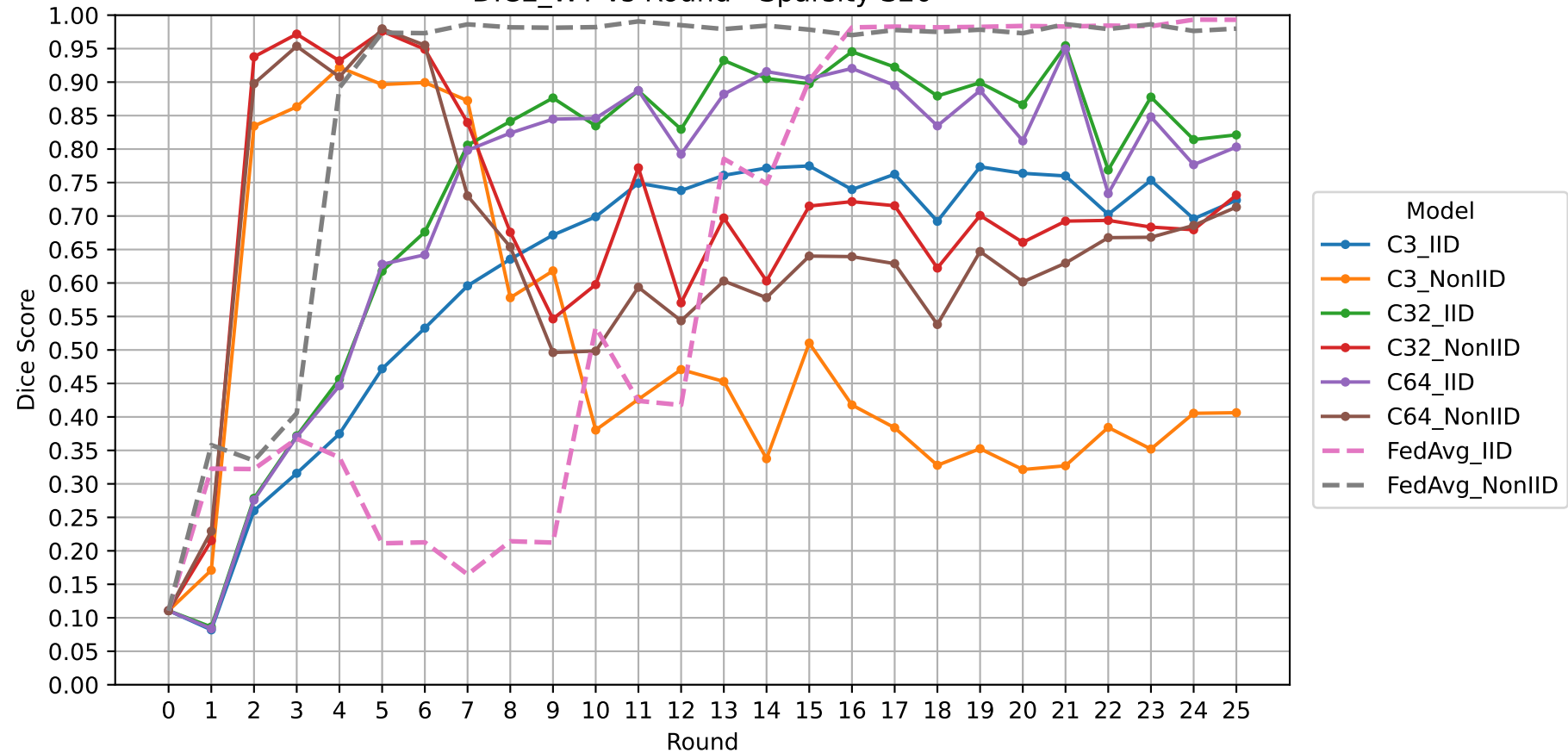
DICE_WT vs Round - Sparsity S20
