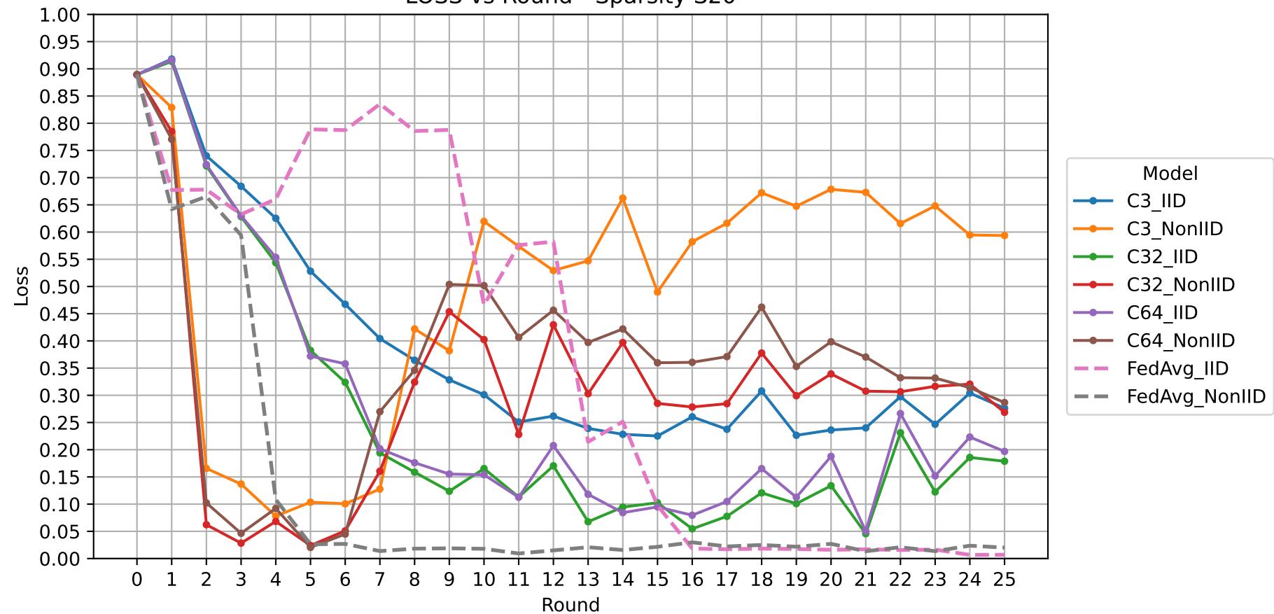
LOSS vs Round - Sparsity S20
