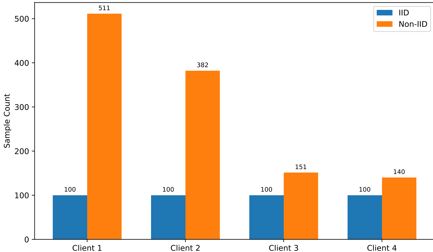
Samples per Client: IID vs Non-IID
