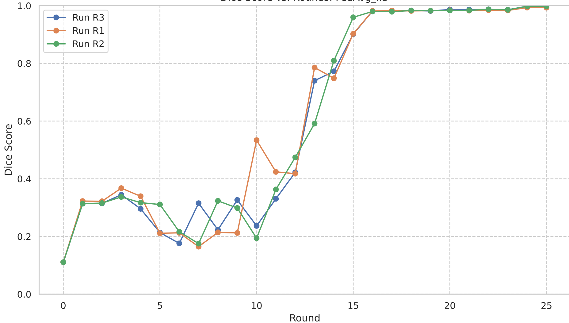
Dice Score vs. Rounds: FedAvg_IID
