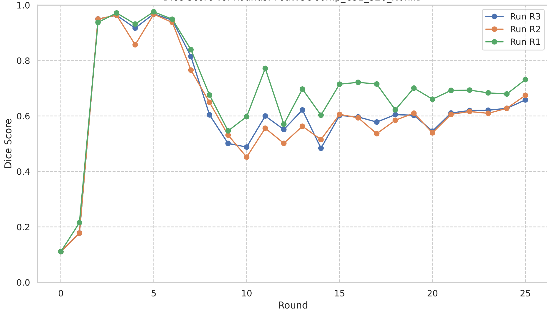
Dice Score vs. Rounds: FedWSOComp_C32_S20_NonIID
